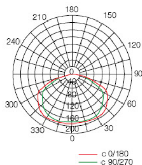
灯具光分布图 Light distribution diagram of lamp
